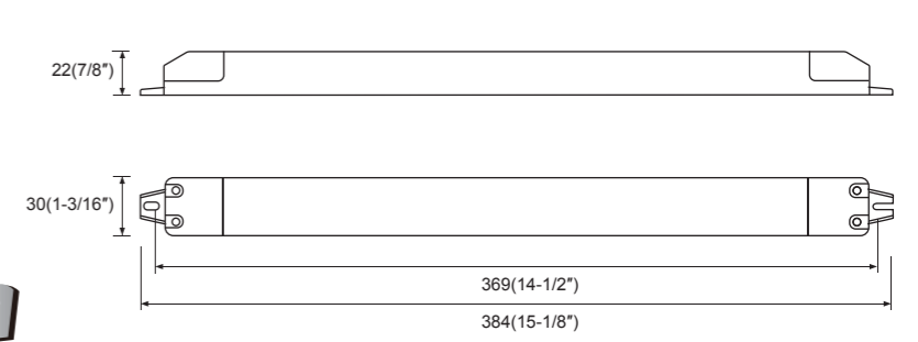
Dimensions: (mm/inch)
