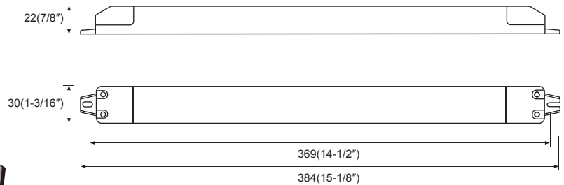
Dimensions: (mm/inch)
